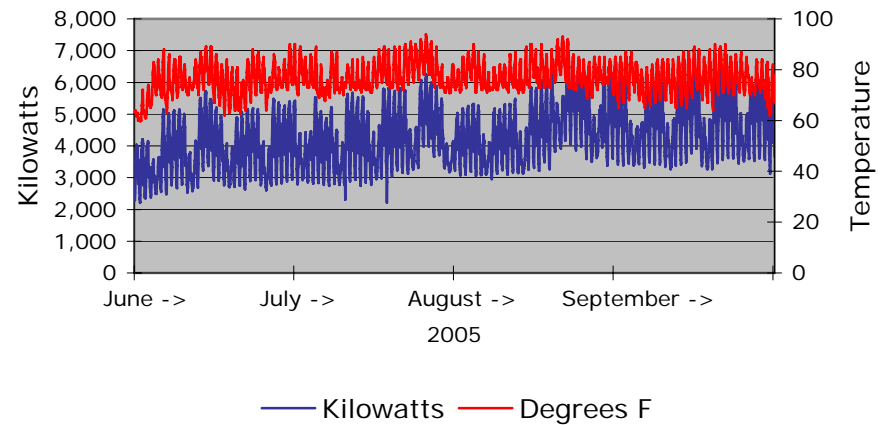
Relationship Between Electric Use and Outside Temperature
